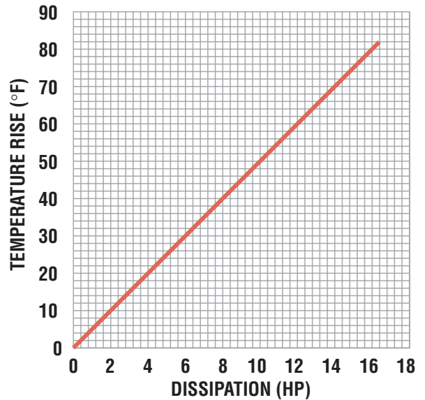
PERFORMANCE CURVE – MH3 HYDRAPAK
