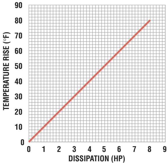
PERFORMANCE CURVE – MH1 HYDRAPAK
